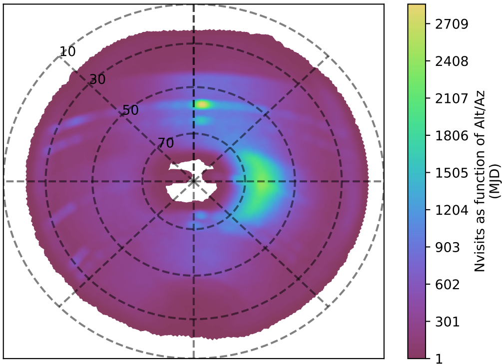
weather_cloudso30v3.4_10yrs i band: Nvisits as function of Alt/Az
