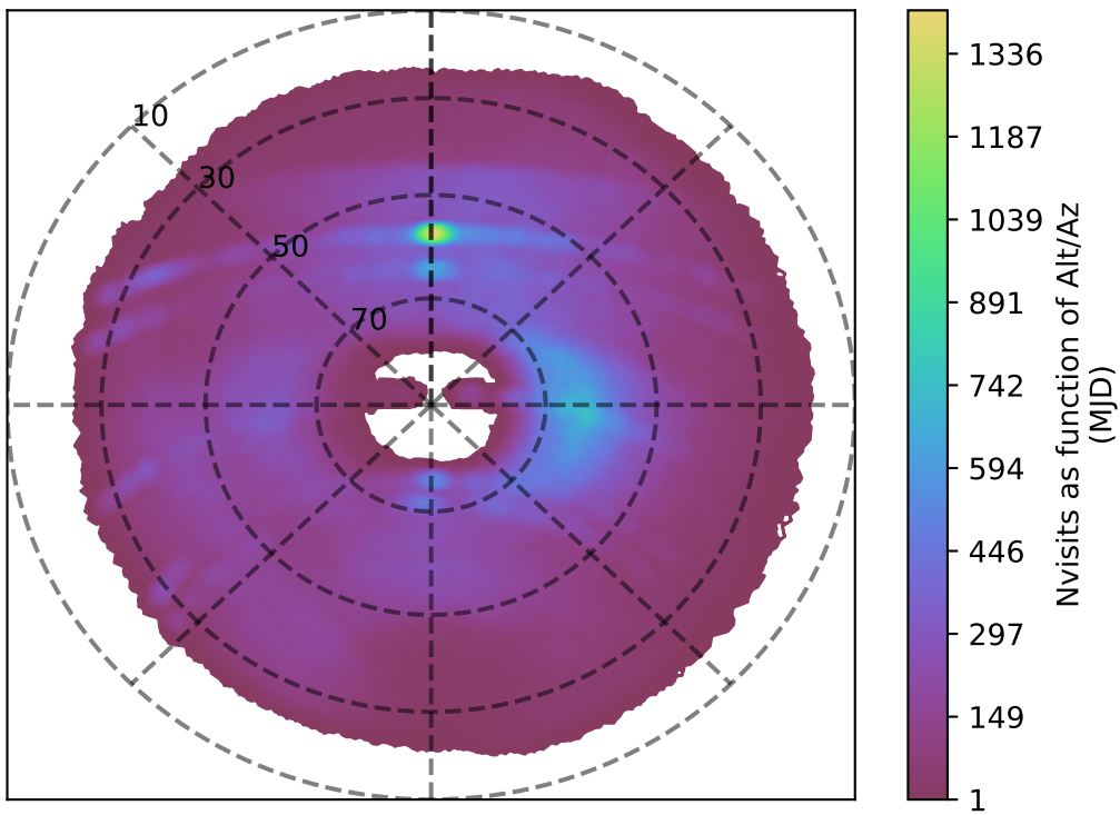
weather_cloudso30v3.4_10yrs g band: Nvisits as function of Alt/Az
