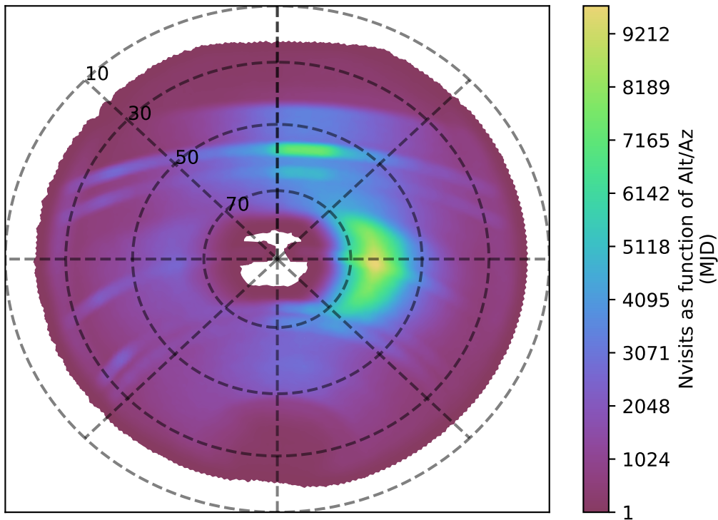
weather_cloudso30v3.4_10yrs all bands: Nvisits as function of Alt/Az
