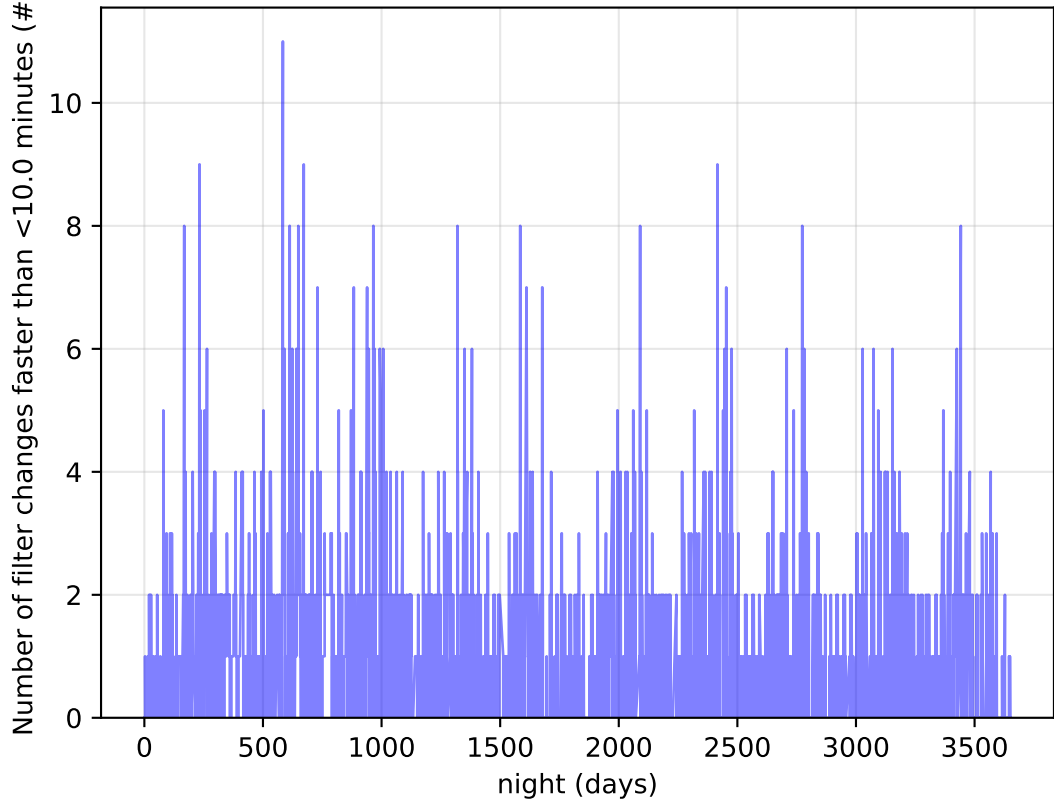
weather_cloudso30v3.4_10yrs Per Night: Number of filter changes faster than <10.0 minutes
