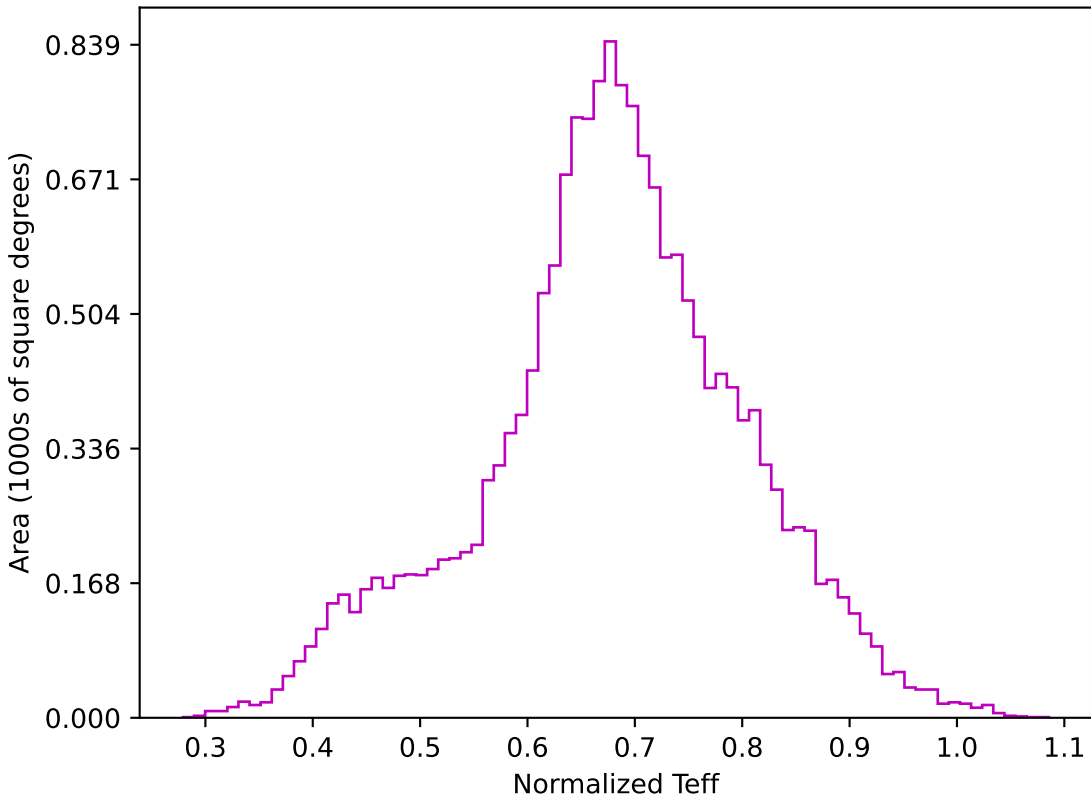
weather_cloudso30v3.4_10yrs WFD z band: Normalized Teff
