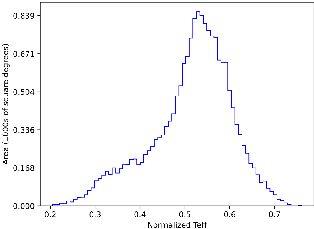
weather_cloudso30v3.4_10yrs WFD y band: Normalized Teff
