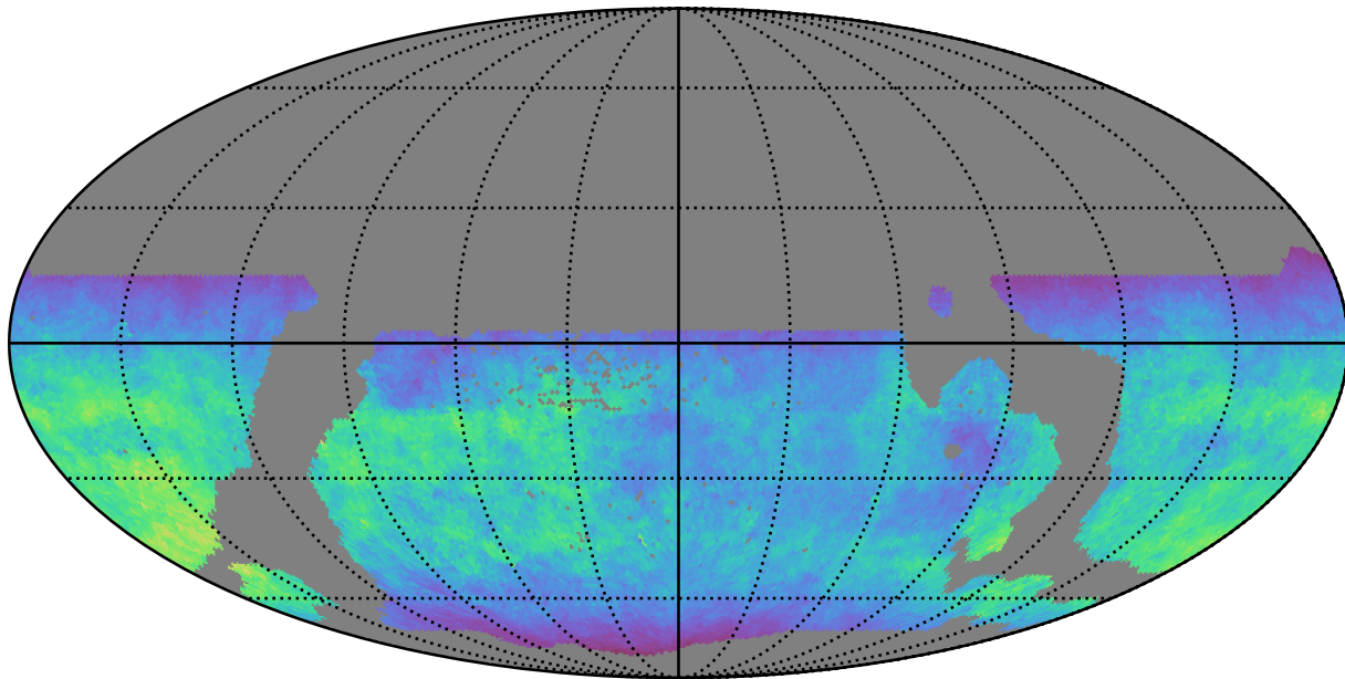
weather_cloudso30v3.4_10yrs WFD u band: Normalized Teff
