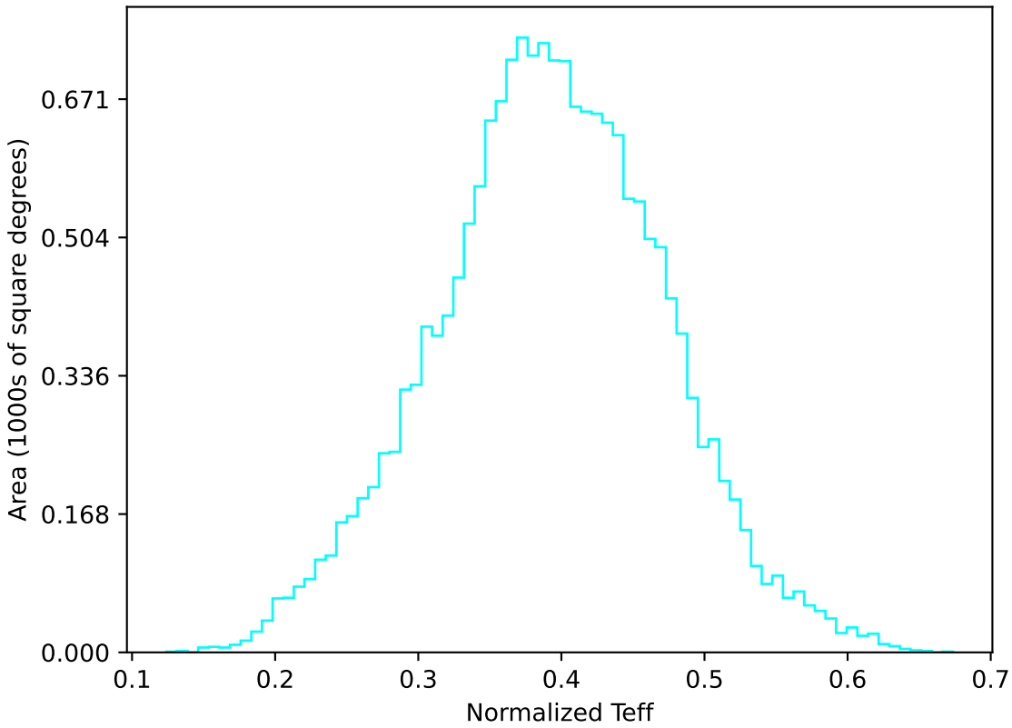
weather_cloudso30v3.4_10yrs WFD u band: Normalized Teff
