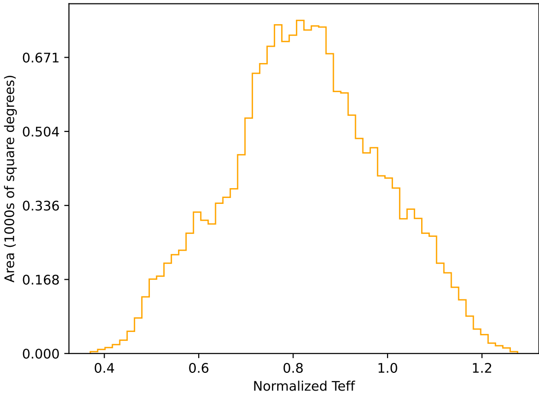
weather_cloudso30v3.4_10yrs WFD r band: Normalized Teff
