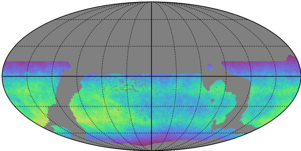
weather_cloudso30v3.4_10yrs WFD i band: Normalized Teff
