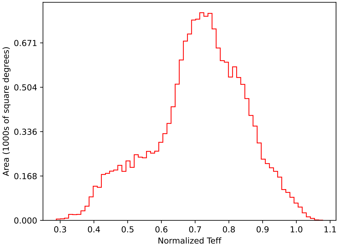
weather_cloudso30v3.4_10yrs WFD i band: Normalized Teff
