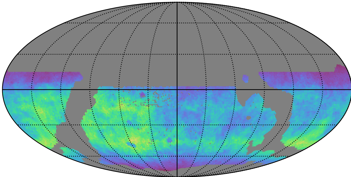
weather_cloudso30v3.4_10yrs WFD g band: Normalized Teff
