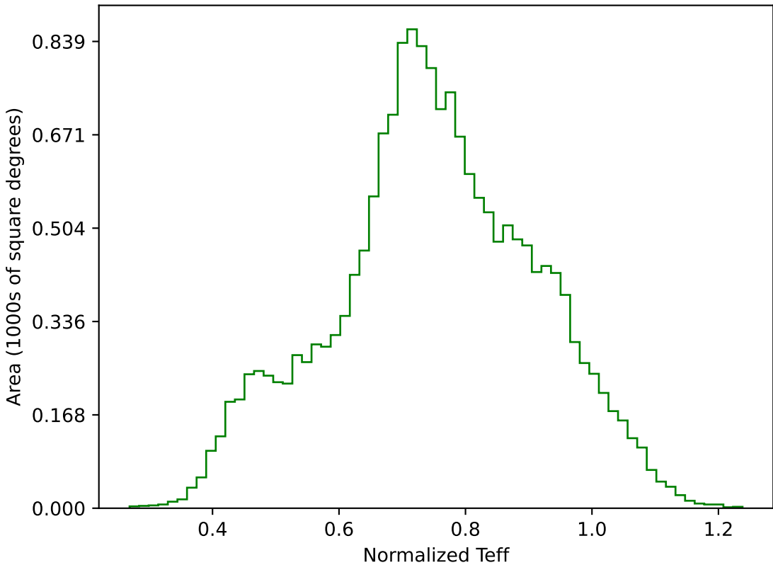
weather_cloudso30v3.4_10yrs WFD g band: Normalized Teff
