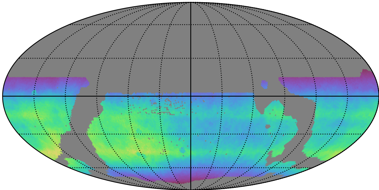
weather_cloudso30v3.4_10yrs WFD all bands: Normalized Teff
