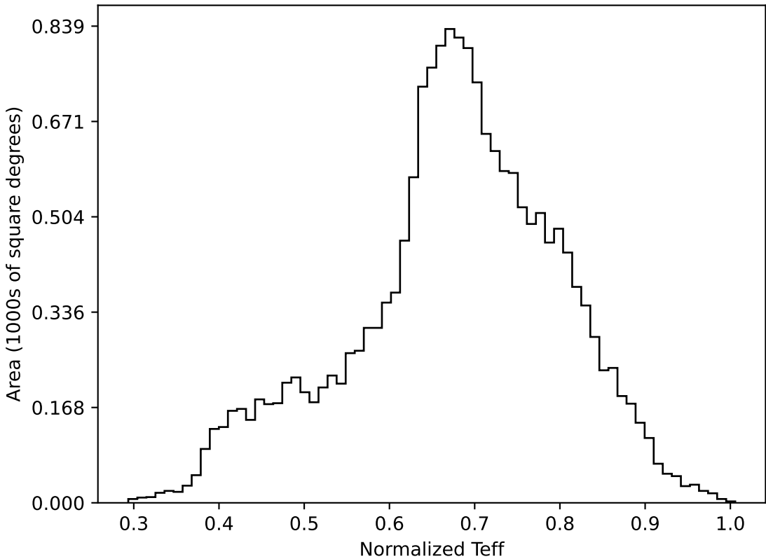
weather_cloudso30v3.4_10yrs WFD all bands: Normalized Teff
