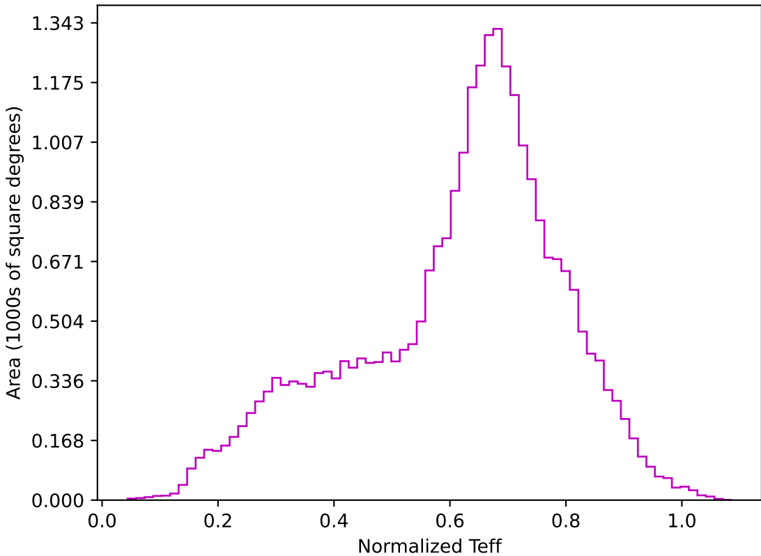
weather_cloudso30v3.4_10yrs All sky z band: Normalized Teff
