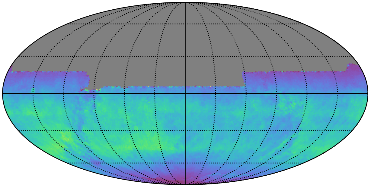
weather_cloudso30v3.4_10yrs All sky y band: Normalized Teff
