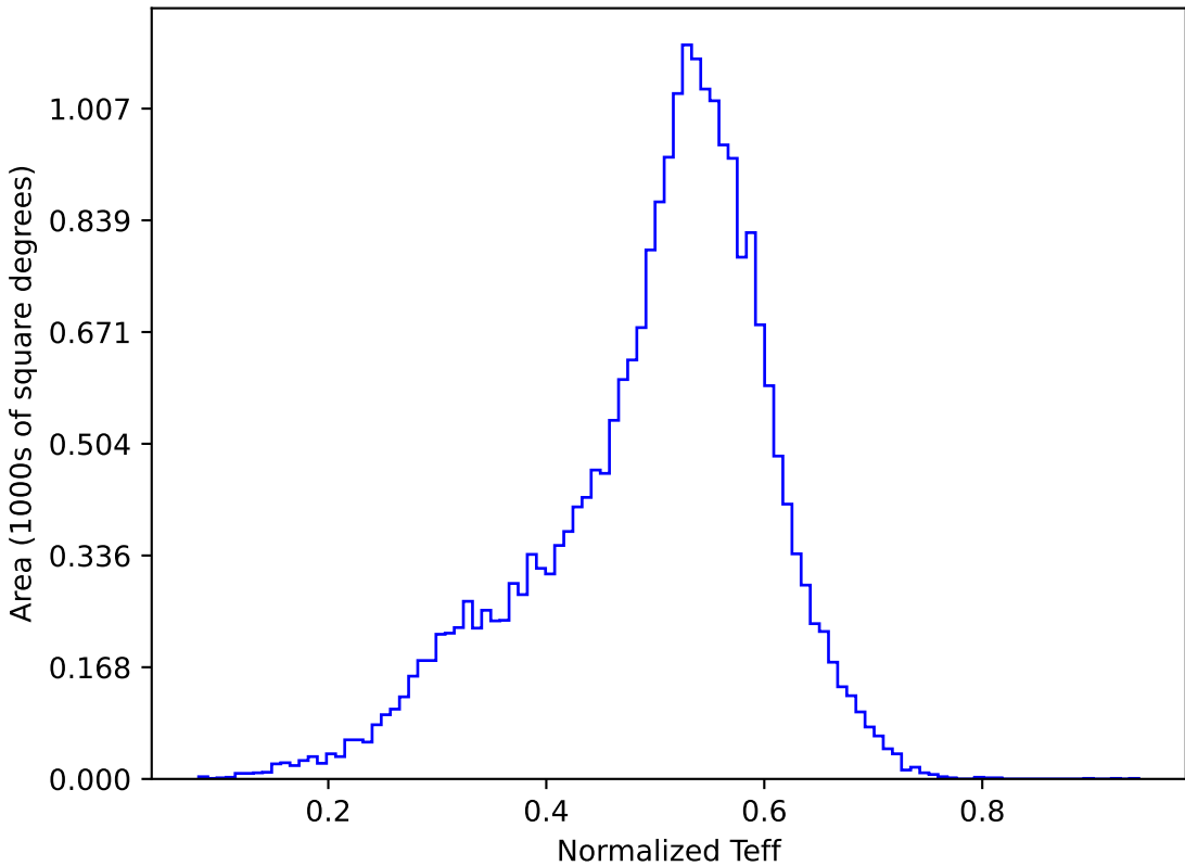
weather_cloudso30v3.4_10yrs All sky y band: Normalized Teff
