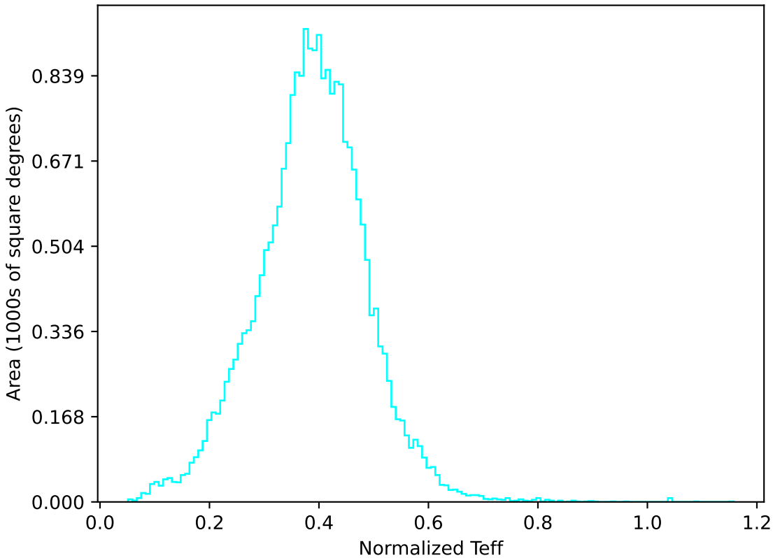
weather_cloudso30v3.4_10yrs All sky u band: Normalized Teff
