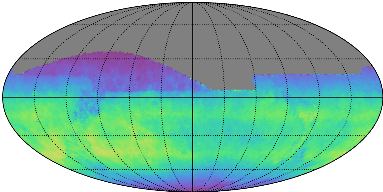
weather_cloudso30v3.4_10yrs All sky i band: Normalized Teff
