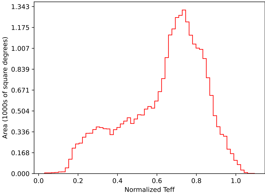
weather_cloudso3v3.4_10yrs All sky i band: Normalized Teff
