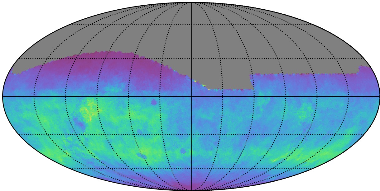
weather_cloudso30v3.4_10yrs All sky g band: Normalized Teff
