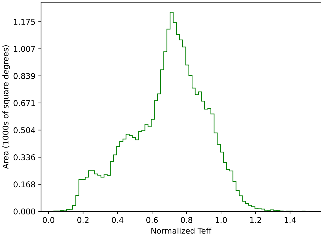
weather_cloudso30v3.4_10yrs All sky g band: Normalized Teff
