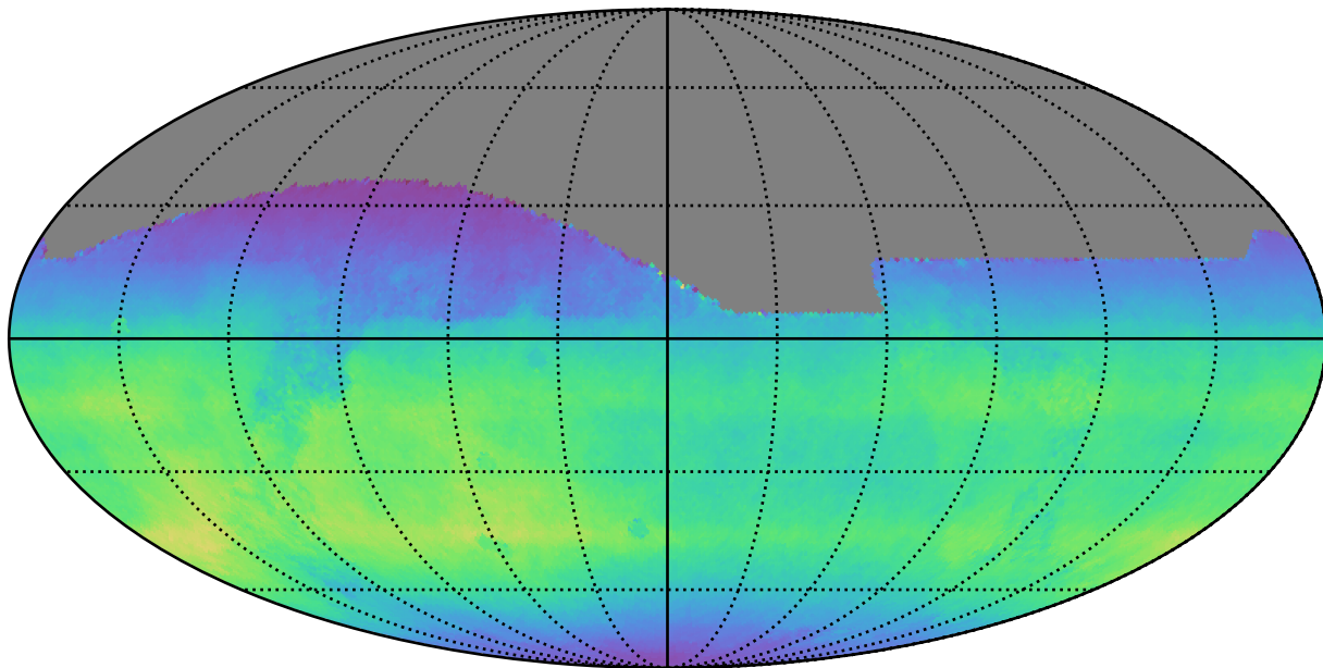
weather_cloudso30v3.4_10yrs All sky all bands: Normalized Teff
