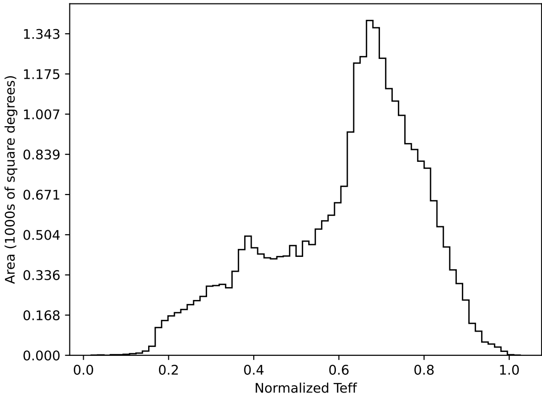
weather_cloudso30v3.4_10yrs All sky all bands: Normalized Teff
