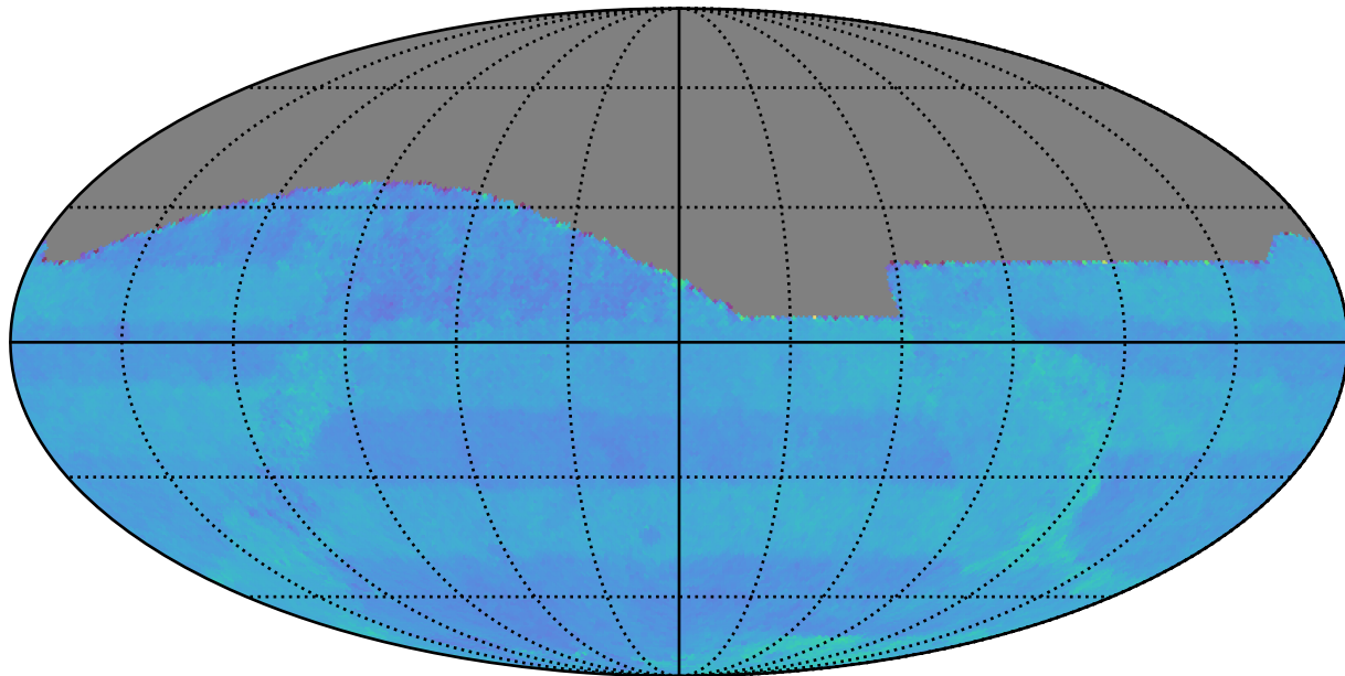
weather_cloudso30v3.4_10yrs All sky: Normalized Proper Motion Uncert @ 24.0
