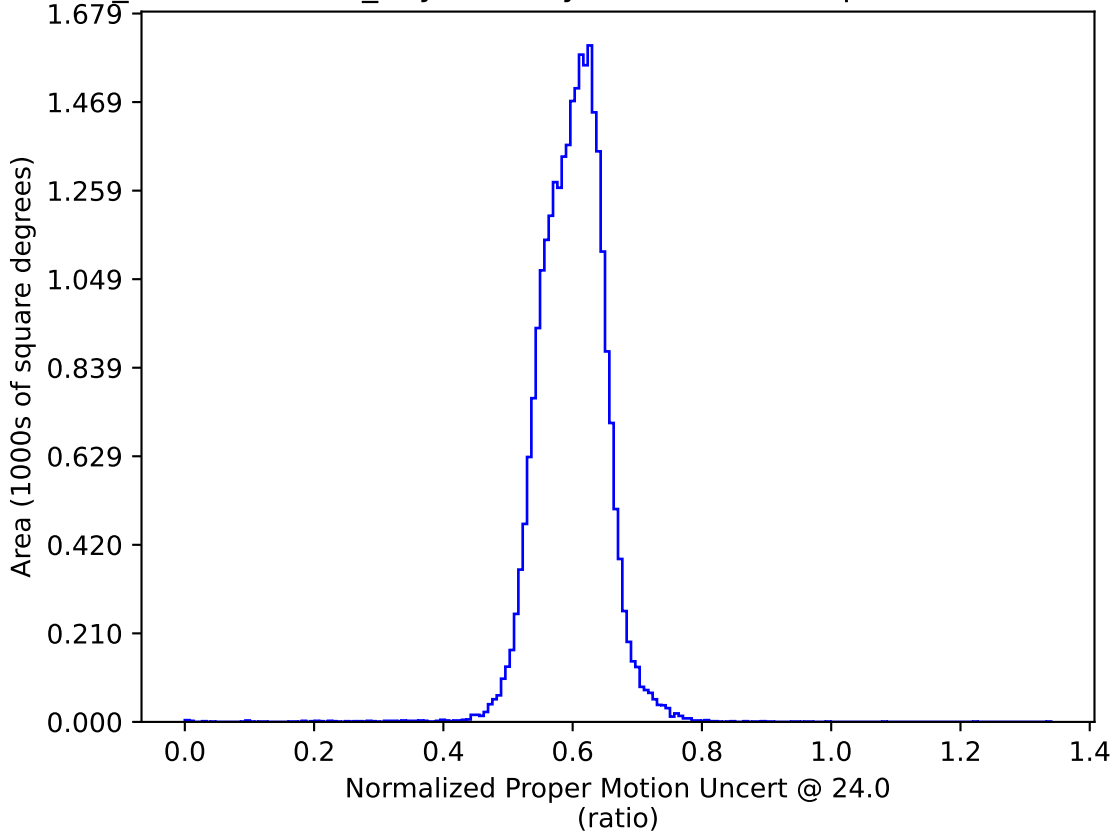
weather_cloudso30v3.4_10yrs All sky: Normalized Proper Motion Uncert @ 24.0
