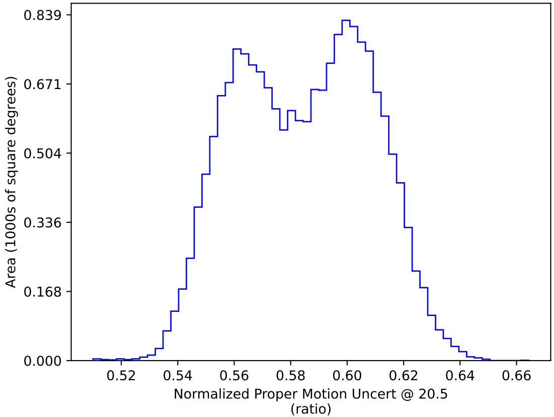
weather_cloudso30v3.4_10yrs WFD: Normalized Proper Motion Uncert @ 20.5
