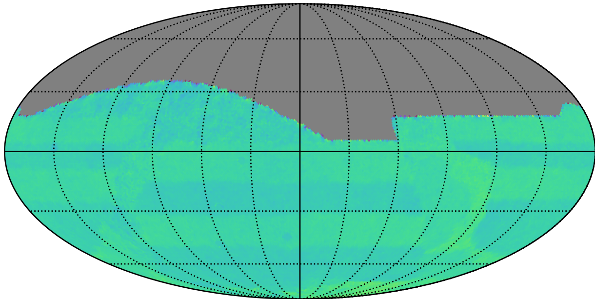
weather_cloudso30v3.4_10yrs All sky: Normalized Proper Motion Uncert @ 20.5
