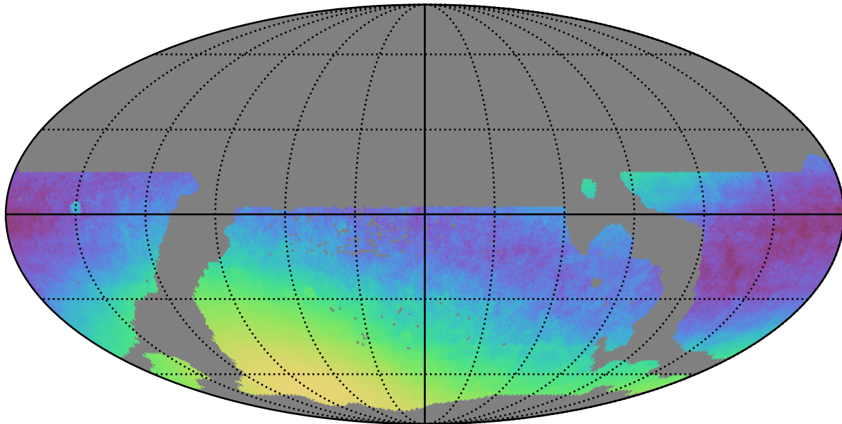
weather_cloudso30v3.4_10yrs WFD: Normalized Parallax Uncert @ 24.0
