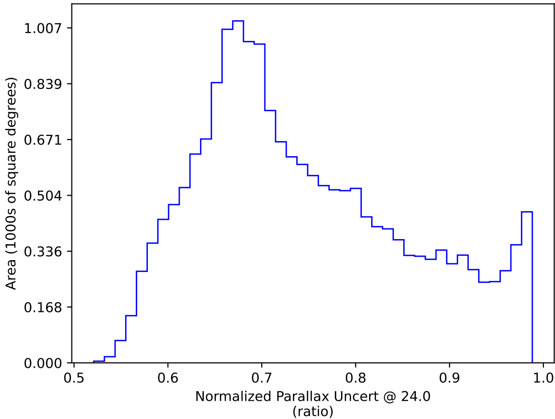
weather_cloudso30v3.4_10yrs WFD: Normalized Parallax Uncert @ 24.0
