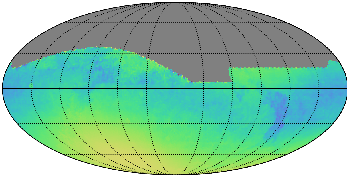
weather_cloudso30v3.4_10yrs All sky: Normalized Parallax Uncert @ 24.0
