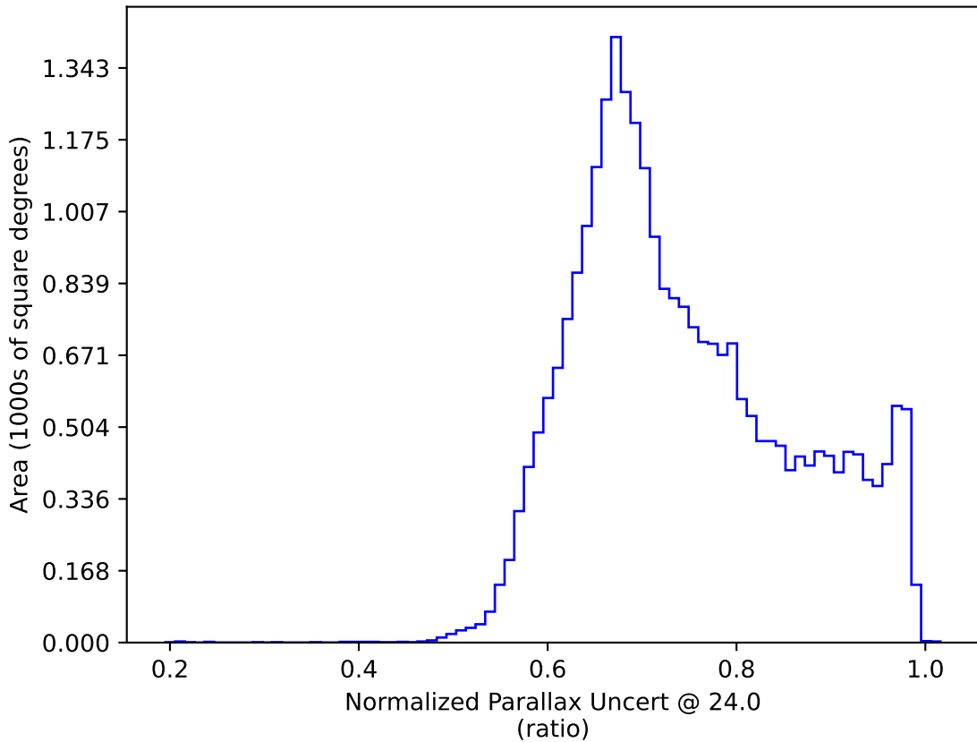
weather_cloudso30v3.4_10yrs All sky: Normalized Parallax Uncert @ 24.0
