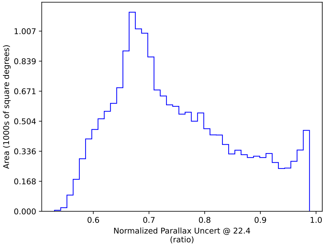
weather_cloudso30v3.4_10yrs WFD: Normalized Parallax Uncert @ 22.4
