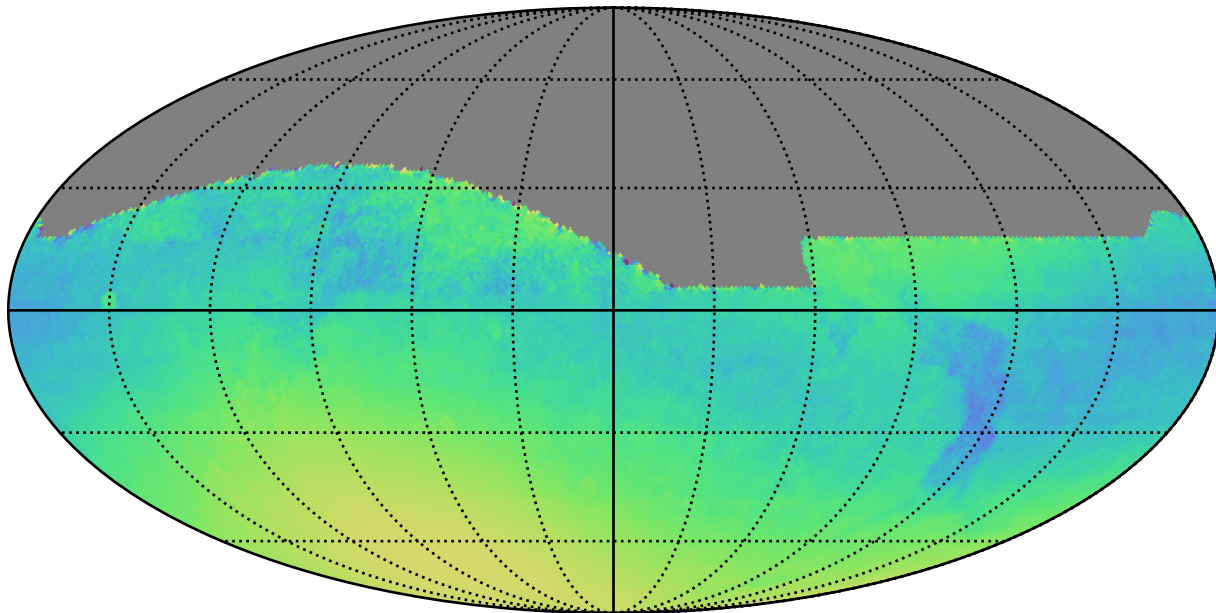
weather_cloudso30v3.4_10yrs All sky: Normalized Parallax Uncert @ 22.4
