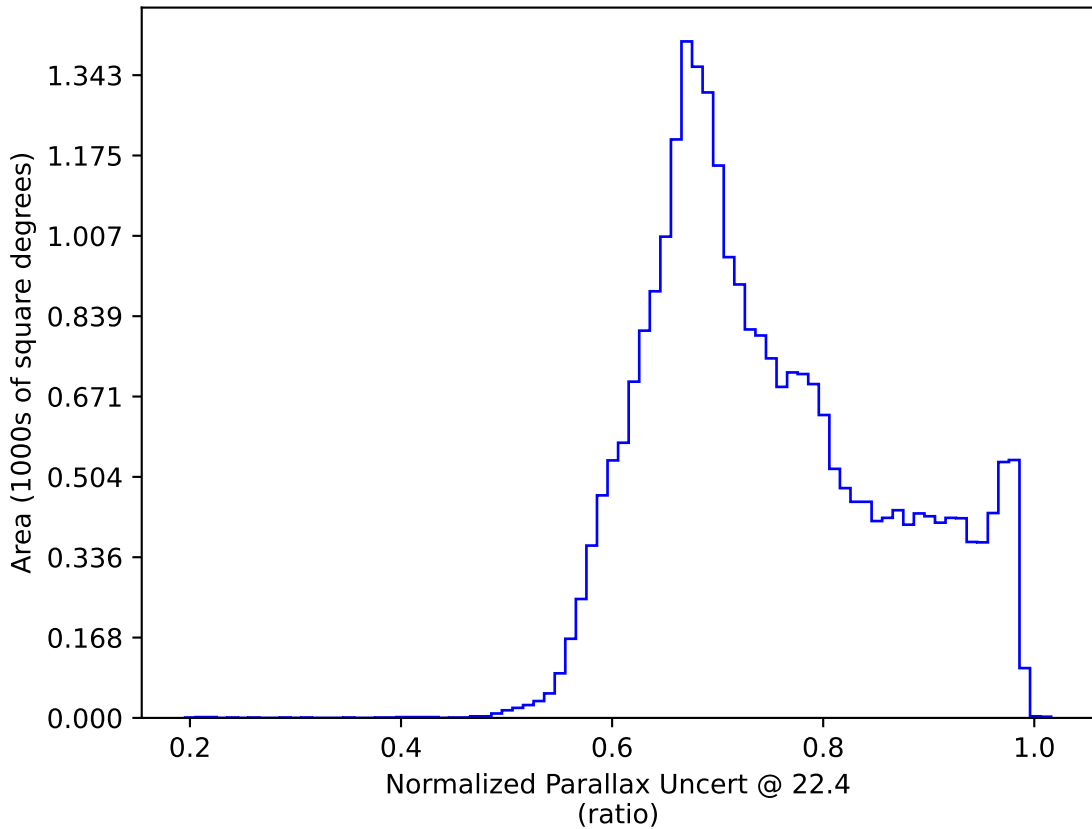
weather_cloudso30v3.4_10yrs All sky: Normalized Parallax Uncert @ 22.4
