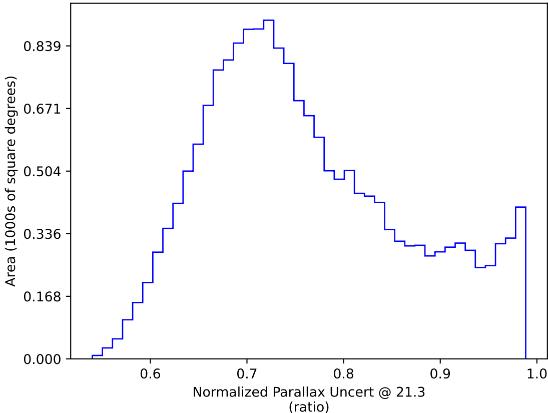
weather_cloudso30v3.4_10yrs WFD y band only: Normalized Parallax Uncert @ 21.3
