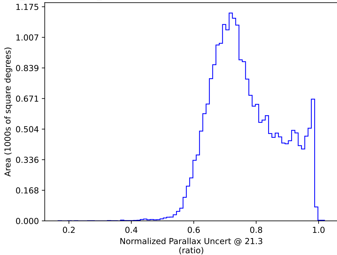
weather_cloudso30v3.4_10yrs All sky y band only: Normalized Parallax Uncert @ 21.3
