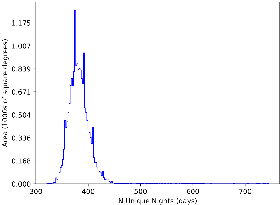
weather_cloudso30v3.4_10yrs WFD all bands: N Unique Nights
