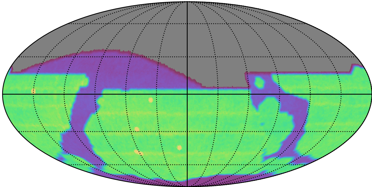
weather_cloudso30v3.4_10yrs All sky all bands: N Unique Nights
