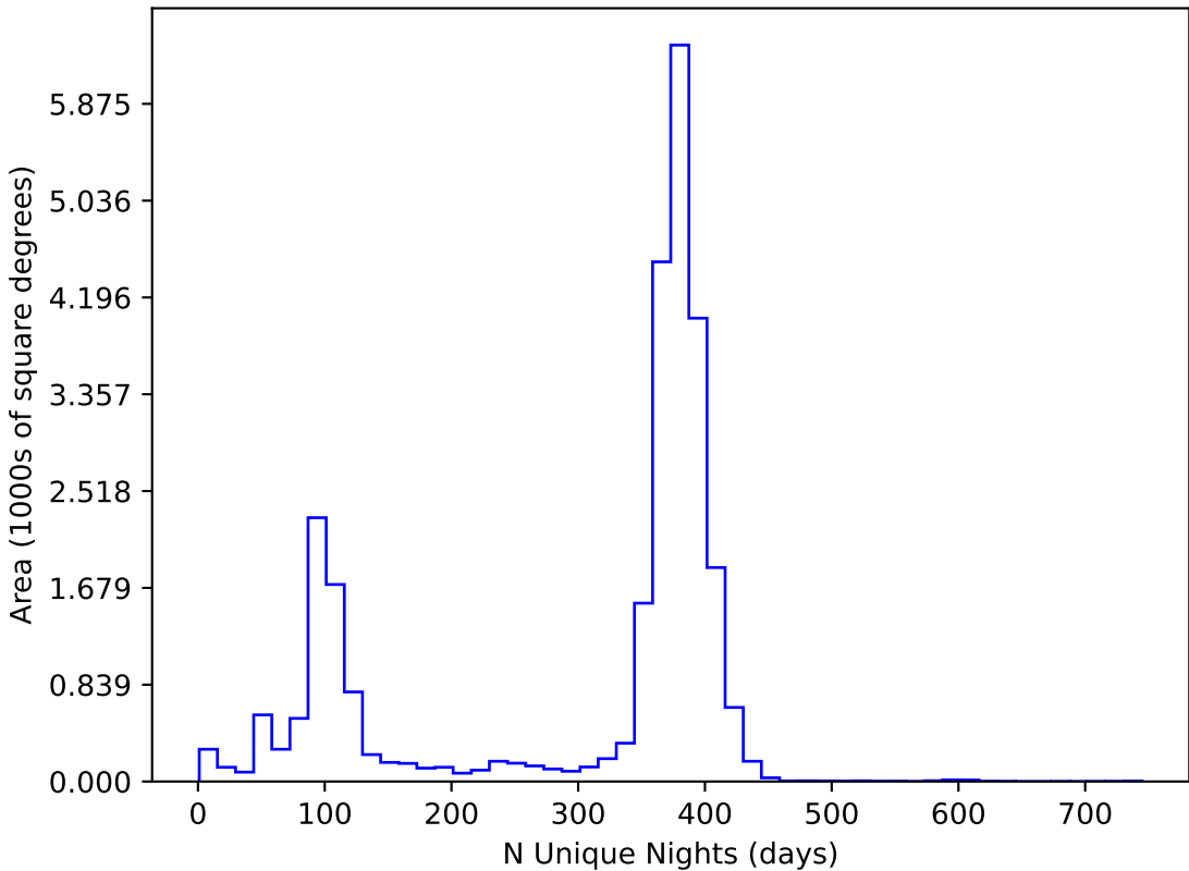
weather_cloudso30v3.4_10yrs All sky all bands: N Unique Nights
