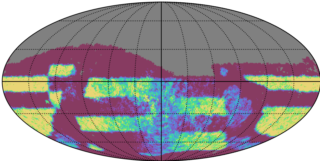
weather_cloudso30v3.4_10yrs Yr 3-4 z band: NVisits
