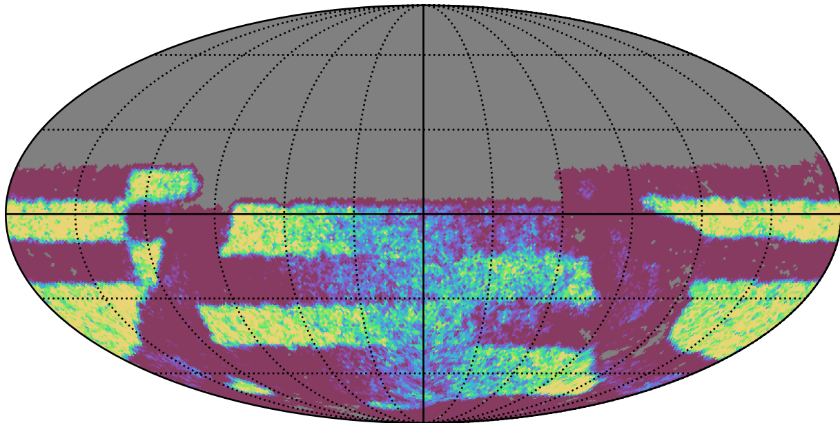
weather_cloudso30v3.4_10yrs Yr 3-4 y band: NVisits
