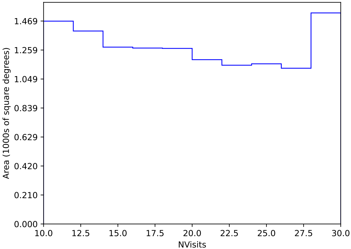
weather_cloudso30v3.4_10yrs Yr 3-4 y band: NVisits
