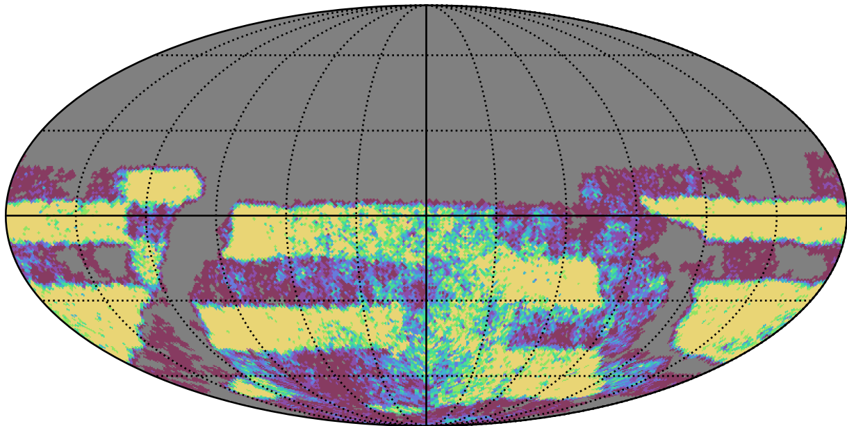
weather_cloudso30v3.4_10yrs Yr 3-4 u band: NVisits
