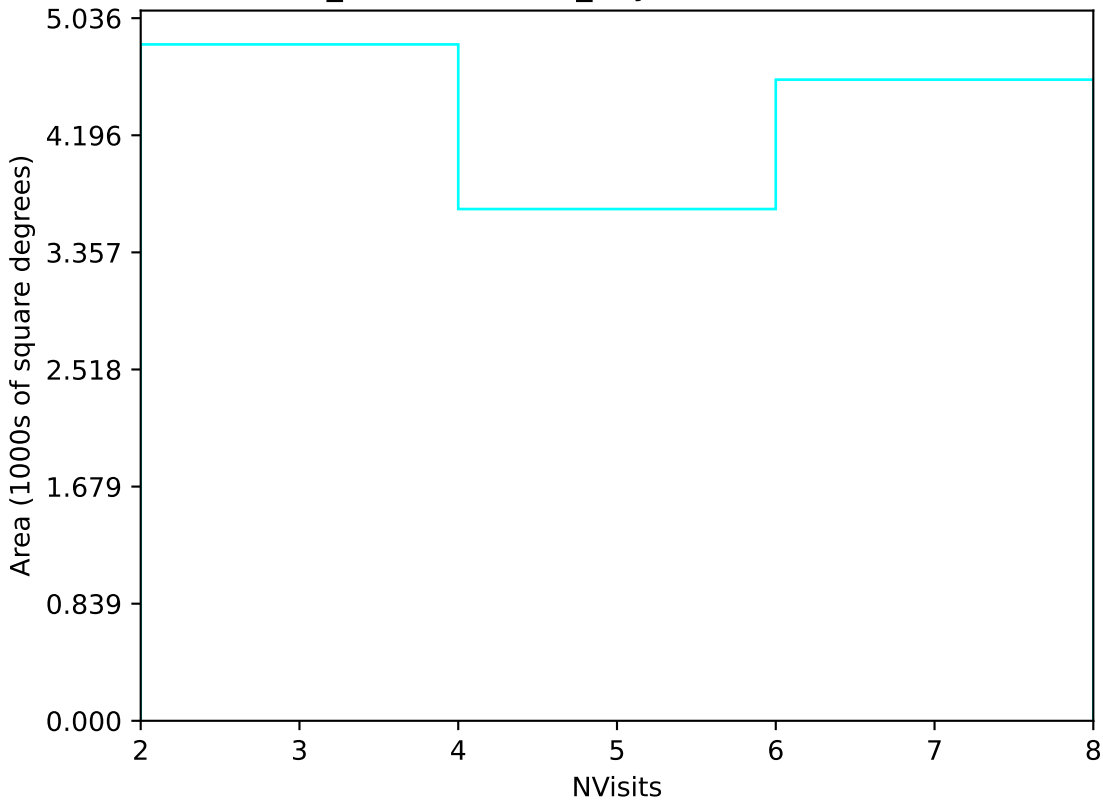
weather_cloudso30v3.4_10yrs Yr 3-4 u band: NVisits
