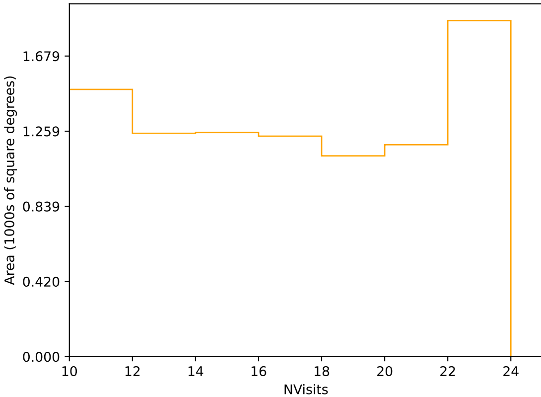
weather_cloudso30v3.4_10yrs Yr 3-4 r band: NVisits
