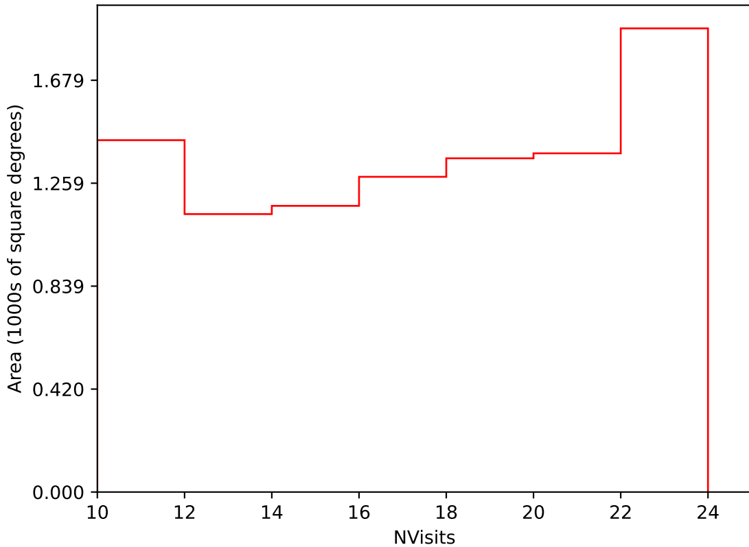
weather_cloudso30v3.4_10yrs Yr 3-4 i band: NVisits
