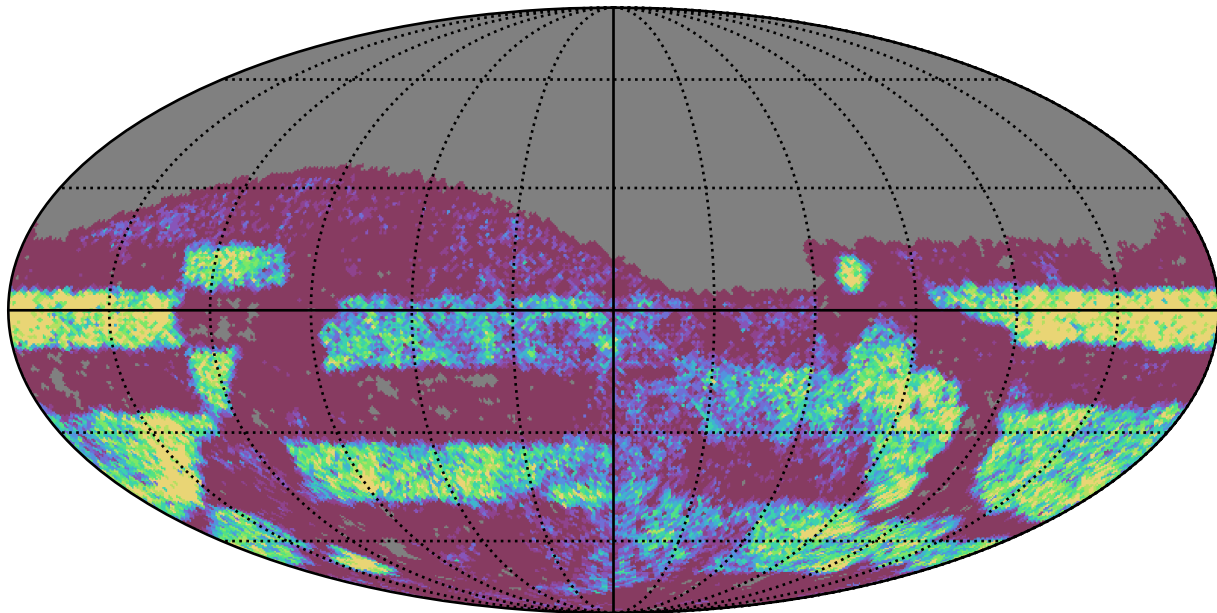
weather_cloudso30v3.4_10yrs Yr 3-4 g band: NVisits
