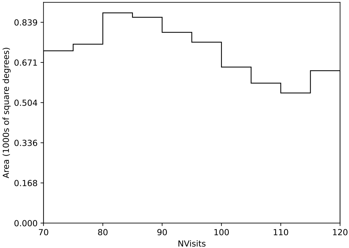
weather_cloudso30v3.4_10yrs Yr 3-4 all bands: NVisits
